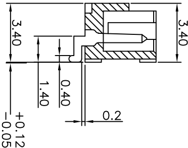
SECT j-j
