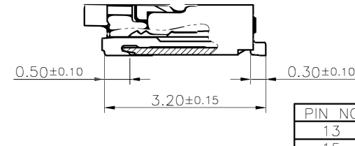
SECTION SCALE 2:1
