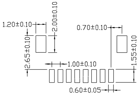
Recommad PCB Layout
